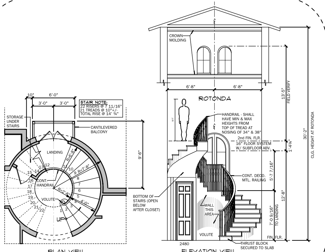
STAIR DETAIL AT ROTONDA SCALE: 1/4" = 1'-0"
