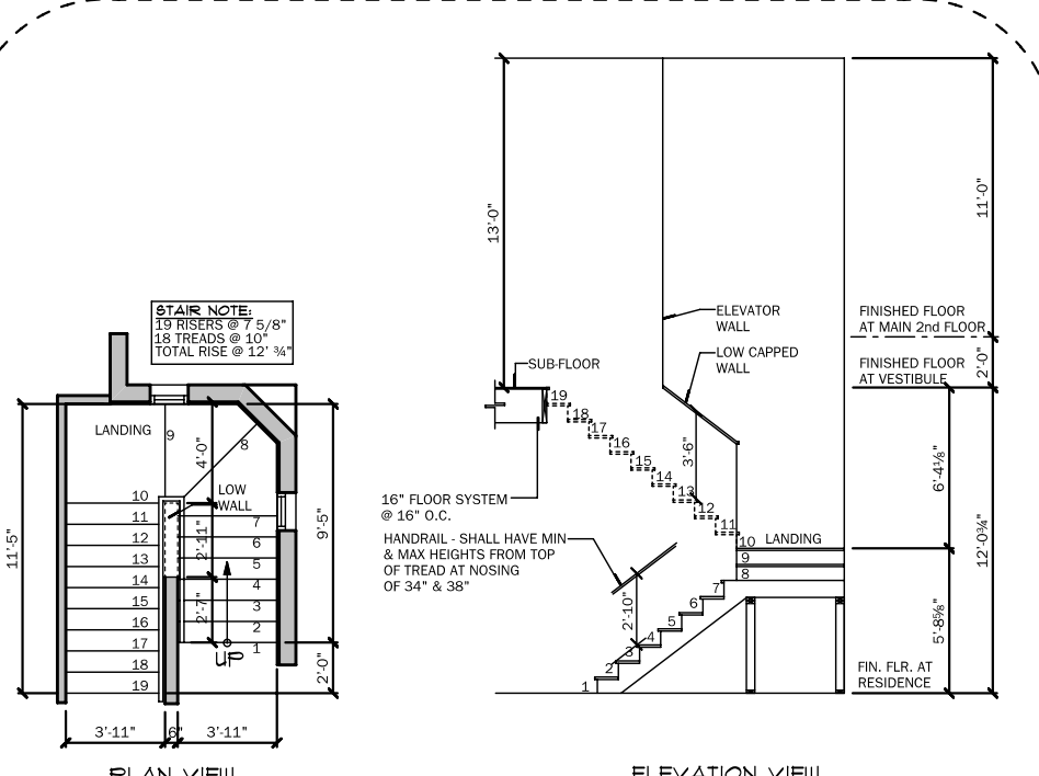
STAIR DETAIL AT 2nd FLOOR VESTIBULE SCALE: 1/4" = 1'-0"
