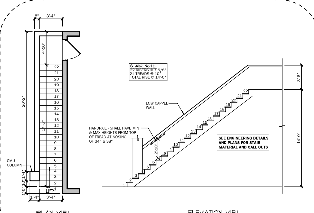
STAIR DETAIL AT COURT YARD SCALE: 1/4" = 1'-0"
