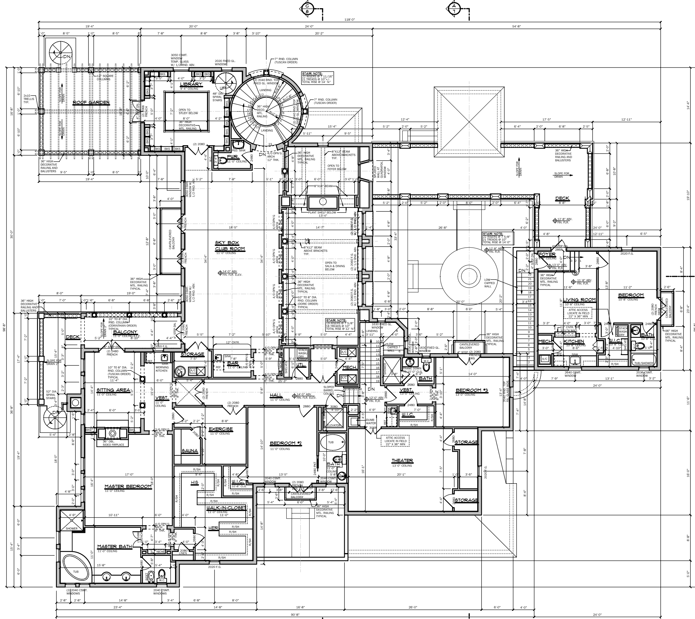
2nd FLOOR PLAN
