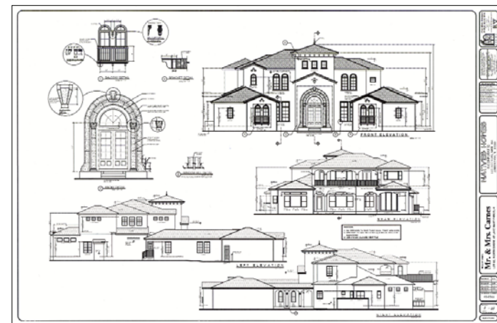
Section details, elevations, and cross sections created in SoftPlan Pro.
