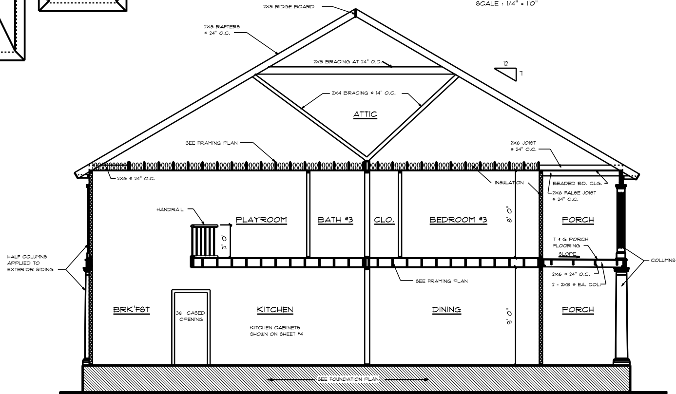
SECTION A SCALE : 1/4" = 1'0"
