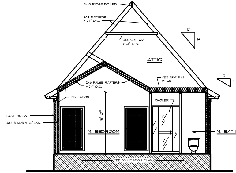
SECTION B SCALE : 1/4" = 1'0"
