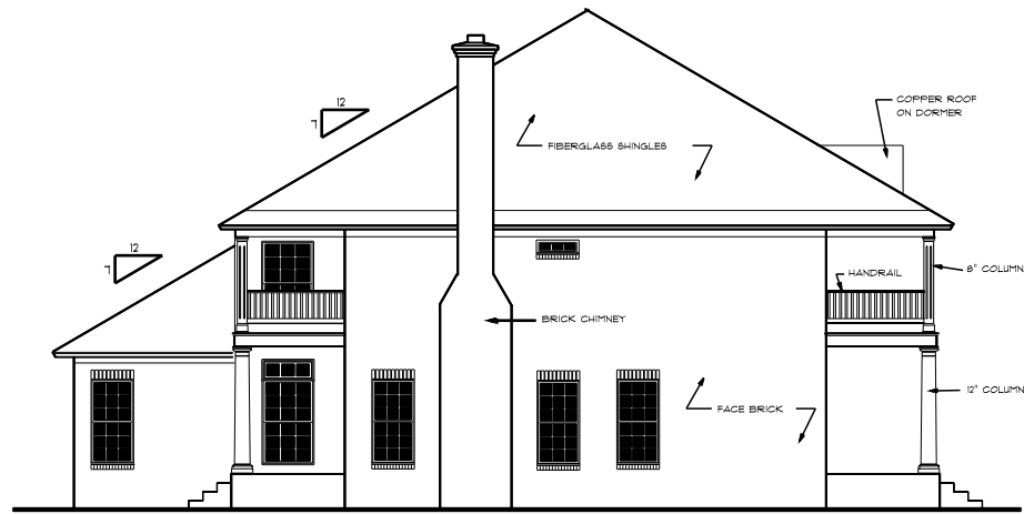
LEFT SIDE ELEVATION SCALE : 1/8" = 1'0"
