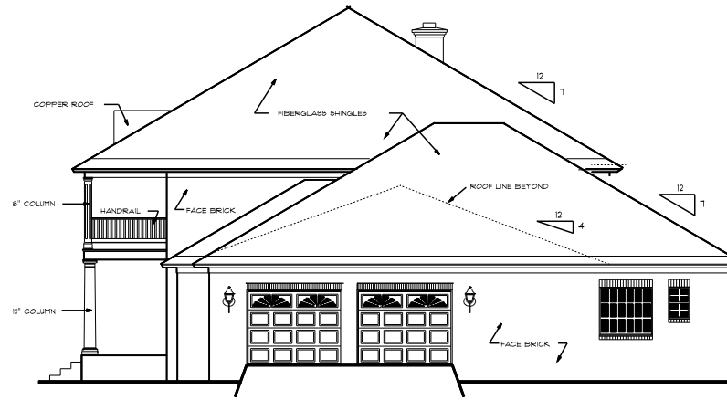
RIGHT SIDE ELEVATION SCALE : 1/8" = 1'0"
